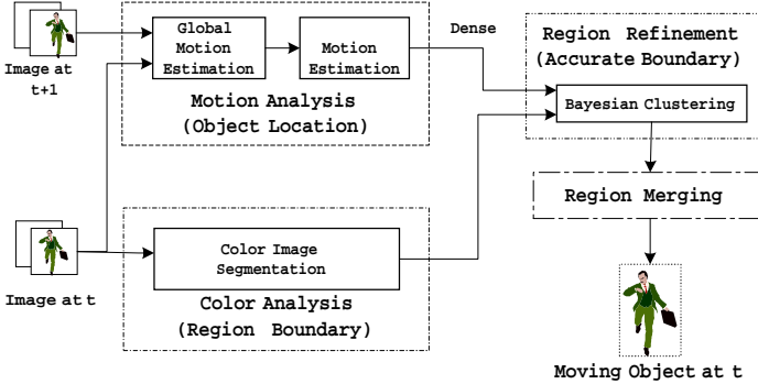
Fig. 1. Proposed Algorithm
