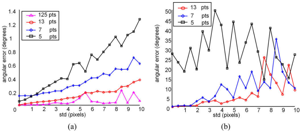
Fig. 9. Simulation results. (a) Error on the estimated rotation angle \theta . (b) Average angular error on the estimated projection rays (angle between estimated and true rays).
