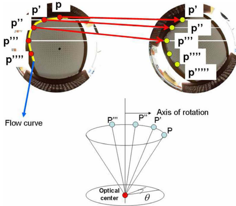
Fig. 2. Illustration of flowcurves from rotational motion ( r -curves). They are formed according to the same principle as outlined in Fig. 1. In the bottom we show the projection rays corresponding to pixels in one r -curve; they lie on a right cone.
