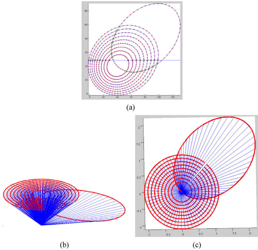
Fig. 8. (a) A few flowcurves associated with two rotations and a single translation are shown, together with fitted conics. (b) and (c) show the metric reconstruction of projection rays observed from two different viewpoints. Note that the projection rays corresponding to translational flowcurves are not shown.
