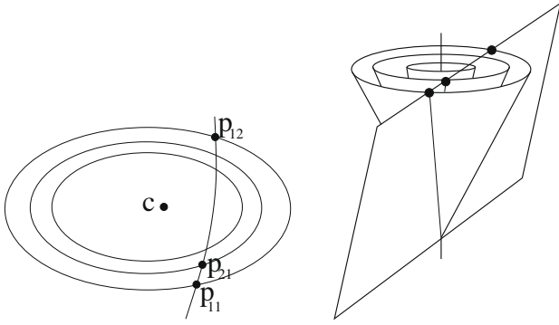
Fig. 5. Computation of the opening angles using a rotation and translation (see text for details).
