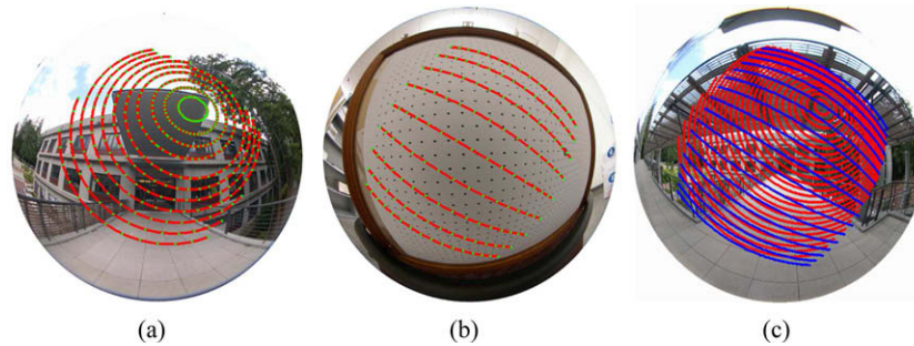
Fig. 10. Flowcurves of a fisheye camera for (a) a pure rotation and (b) a pure translation. (c) Intersection of translation and rotational flowcurves.
