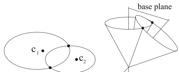
Fig. 6. Computation of the azimuth angles from two rotations (see text for details).
