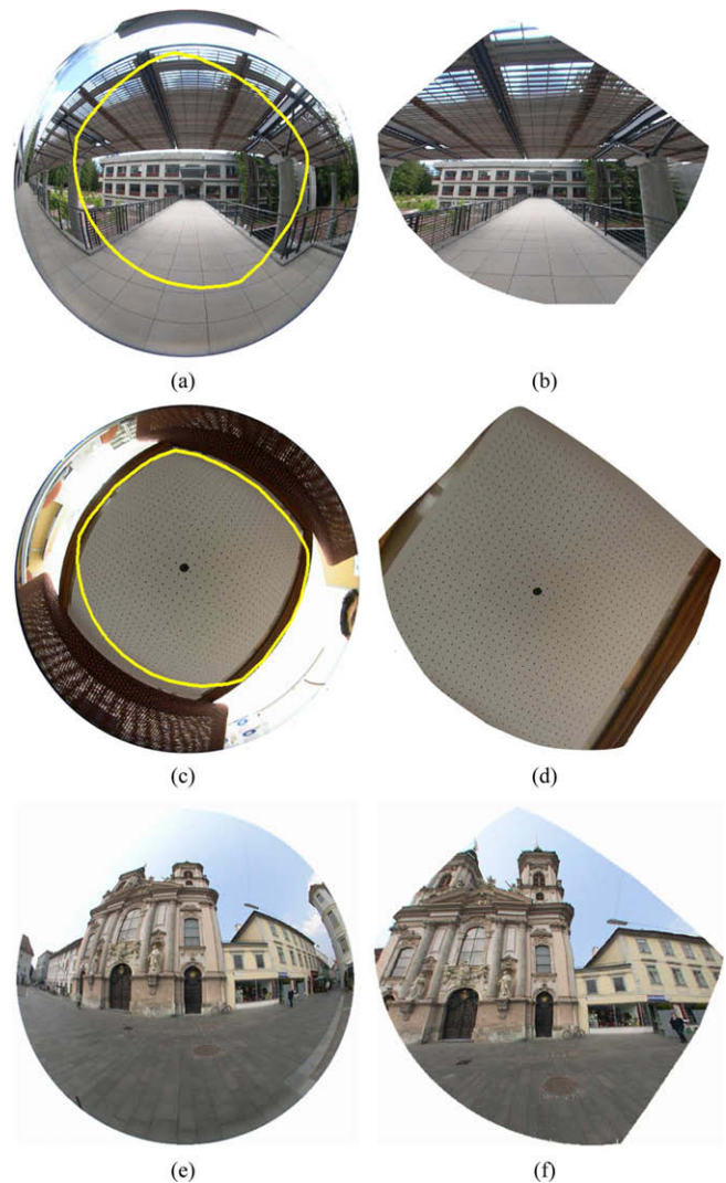
Fig. 11. We show the original images along with the boundary showing the calibrated region on the left. On the right we show the distortion correction for the calibrated region.
