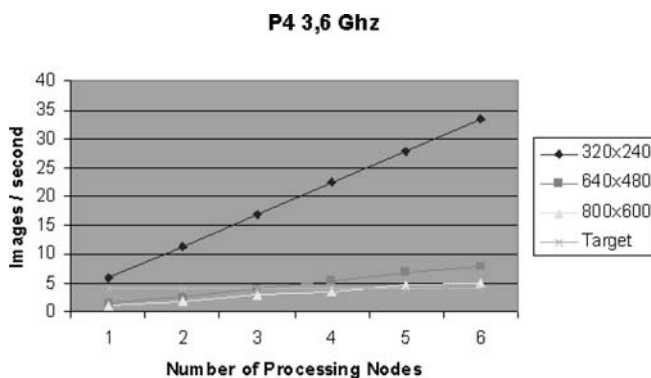
Fig. 12 Performance for different image resolutions (target 4 img/s)
