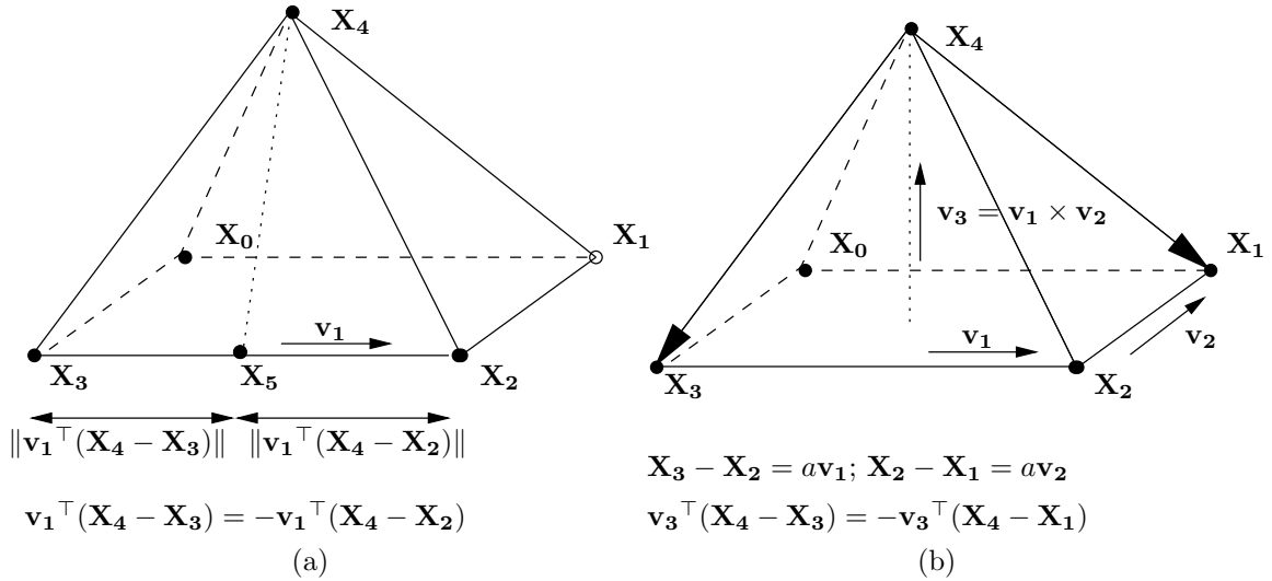
Figure 1.9: Examples of using known scene directions to impose euclidean constraints: symmetry, distances and distance ratios: (a) Symmetry of vectors X_5X_3 and X_5X_2 with respect to plane perpendicular to both vectors and passing through X_5 : projections of vectors X_3X_4 and X_4X_2 on direction v_1 have the same length; (b) Symmetry of vectors X_4X_3 and X_4X_1 : projections of vectors X_1X_4 and X_3X_4 on direction v_3 have the same length. Distances: known distances on lines with known directions give linear constraints in terms of unknown points X_1, X_2, X_3 . When only the distance ratio is known, the expression remains linear in terms of unknown points and distance a .
