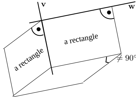
Figure 4.2: Illustration of the case of two right angles.
