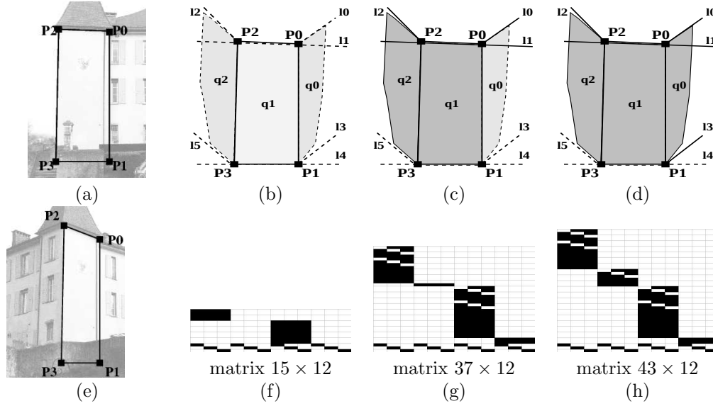
Figure 6.3: Illustration of the reconstruction process. 1st column: fragments of the original images with marked interest points. P1, P3 are occluded in all images. 2nd, 3rd, 4th column: the constraints influencing the interest points. 1st row: the relations between the considered objects. Lines and planes which can influence the interest points P1 - P3 (their coordinates are reconstructed at this step) are marked with black continuous line (lines) or in dark gray (planes); 2nd row: the corresponding constraint matrices. Black fields correspond to non-zero matrix elements.
