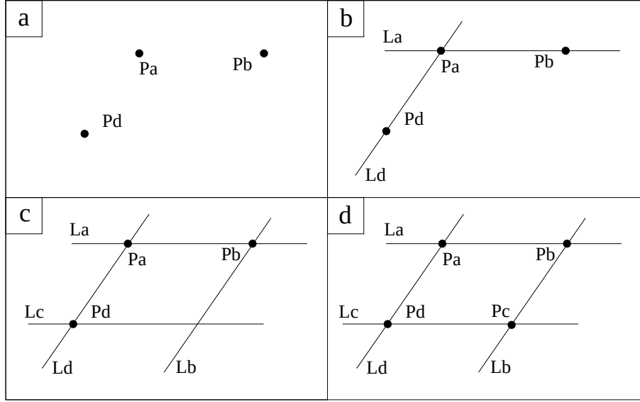
Figure 8.3: Execution of r-methods in the plan ( m_1, m_7, m_3, m_5, m_4 ). (a) The input parameters (i.e., coordinates of P_a , P_b and P_d ) are replaced by their current value. (b) m_1 and m_7 place lines L_a and L_d resp. (c) m_3 and m_5 place L_b and L_c resp. (d) Finally, m_4 places point P_c .
