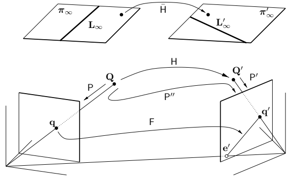
Figure 2. Camera settings. \mathbf{P} is the perspective projection matrix from the first basis to the first reference camera and \mathbf{P}' from the second basis to the second reference camera. \bar{\mathbf{P}}'' is the projection matrix of the second reference camera expressed in the first basis, i.e. it projects points expressed in the first basis in the second reference camera. \mathbf{P} and \mathbf{P}' are assumed known while \bar{\mathbf{P}}'' , which depends on the motion parameters, is unknown. These settings can be easily transposed to the affine, metric and Euclidean cases.
