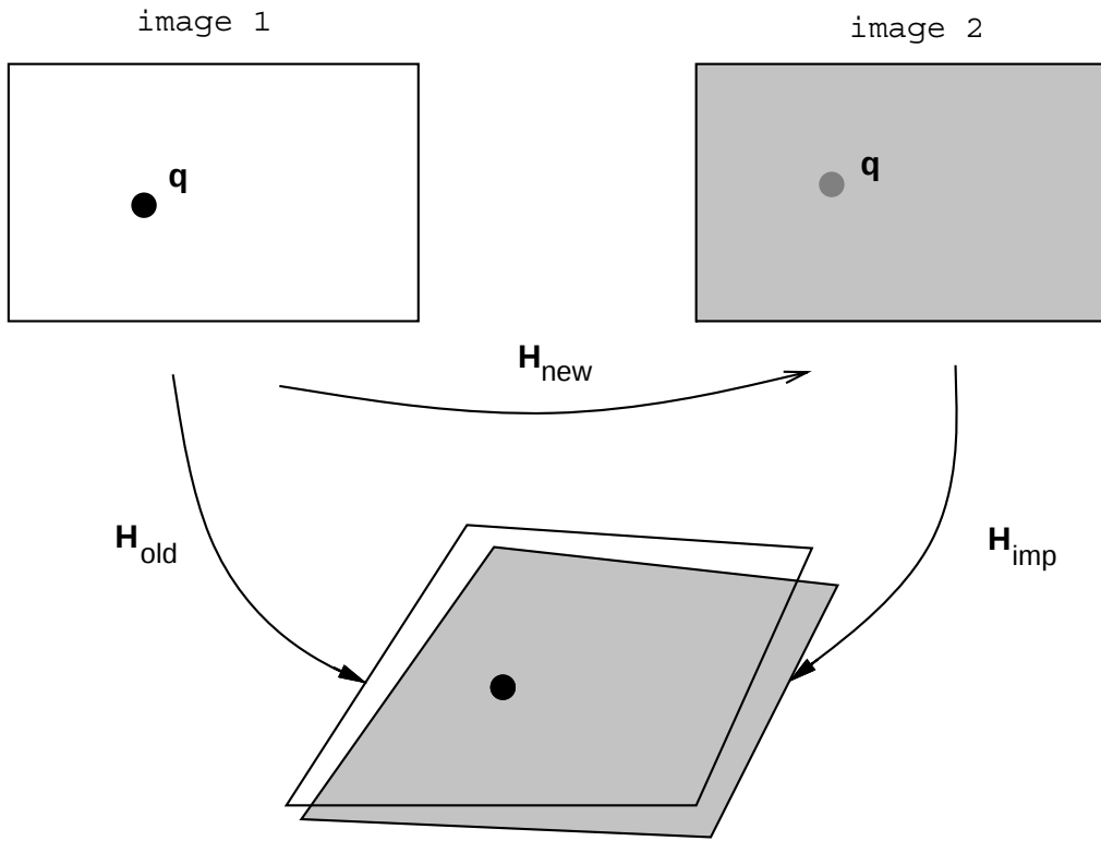
Figure 3: Incremental estimation of the homography between two images. This figure shows the factorisation of H_{\text{old}} into two matrices, H_{\text{imp}} and H_{\text{new}} . This factorisation allows a simpler and faster iterative estimation of the homography by the direct method.
