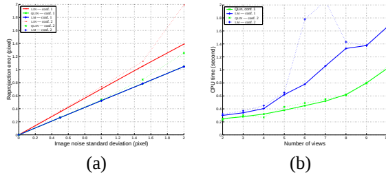
Figure 1. (a): reprojection error at convergence versus added image noise. The curves for QLIN and LM and the first configuration, and for LM and the second configuration are nearly undistinguishable. (b): CPU time to convergence versus the number of views.
