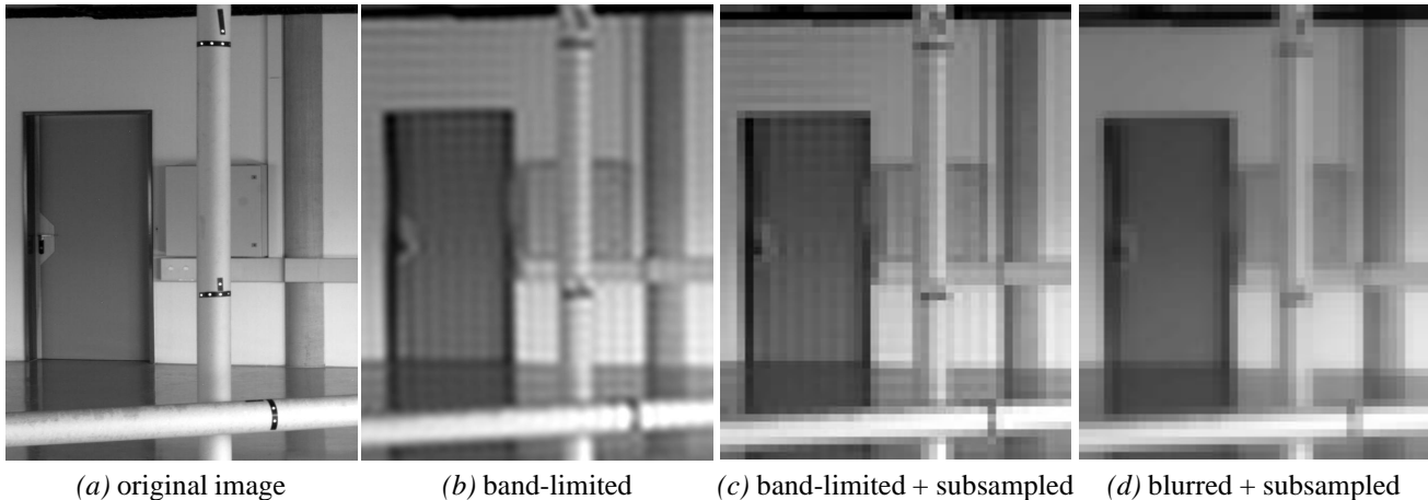
Figure 1: The effects of abrupt bandwidth limitation. An original image (a), limited to 1/15 of the bandwidth (b) then decimated (point-subsampled) 15\times (c). The band-limited images (b,c) have characteristic “ringing” artifacts: Nyquist frequency waves propagate outwards from each edge making smooth surfaces look striped or plaided, especially between parallel edges. Blurring (a) with a \sigma = 7 Gaussian before subsampling gives a slightly less sharp image (d), but no ringing.
