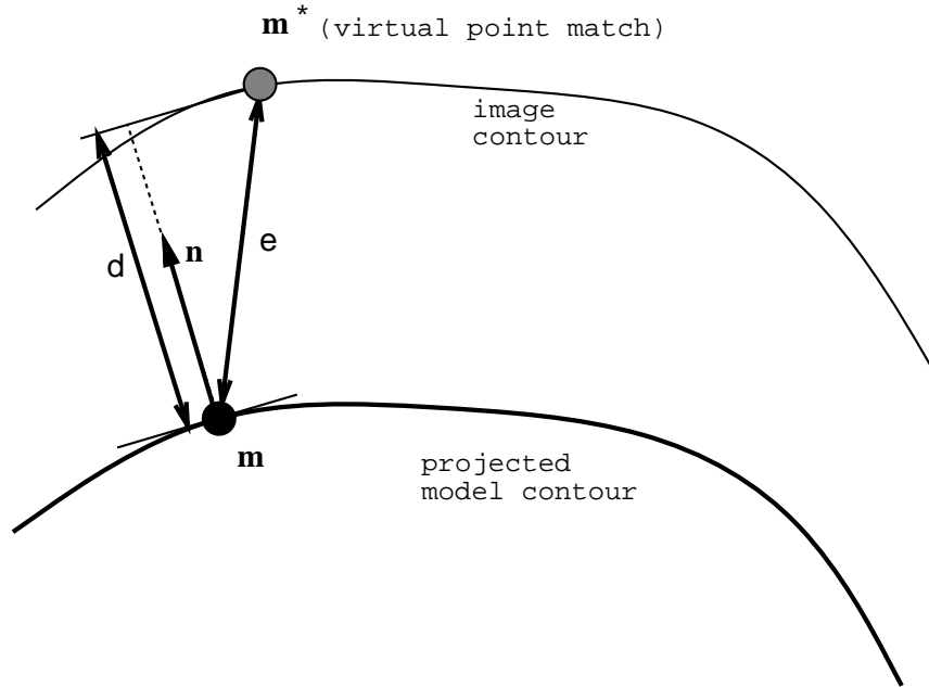
Figure 1: A model contour is predicted in the image and a point location \mathbf{m} along this contour is considered. For point-to-point correspondences, it is sufficient to search for a matching point \mathbf{m}^* end to determine the distance e between these points. For point-to-contour correspondences the strategy consists of raising a normal to the model contour at location \mathbf{m} , finding the intersection of the line supporting the normal vector with the matching image contour, and determining the distance from \mathbf{m} to the image contour. The algebraic expression of this true point-to-contour distance can be approximated by d = \mathbf{n} \cdot (\mathbf{m}^* - \mathbf{m}) .
