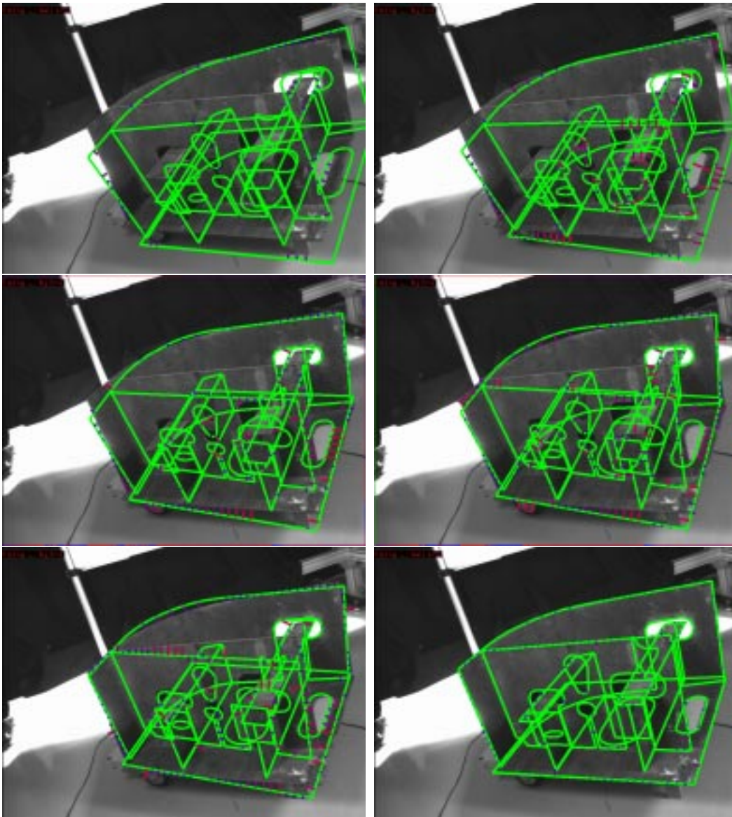
Figure 5: This figure shows an object location example from initialization to convergence. 18 iterations were necessary in this case. The figure shows (left to right and top to down) the initialization, as well as iterations 3, 6, 9, 12, and 18. Although the algorithm performs hidden-line elimination and considers only the model points predicted visible, the display shows all (visible and hidden) model edges.
