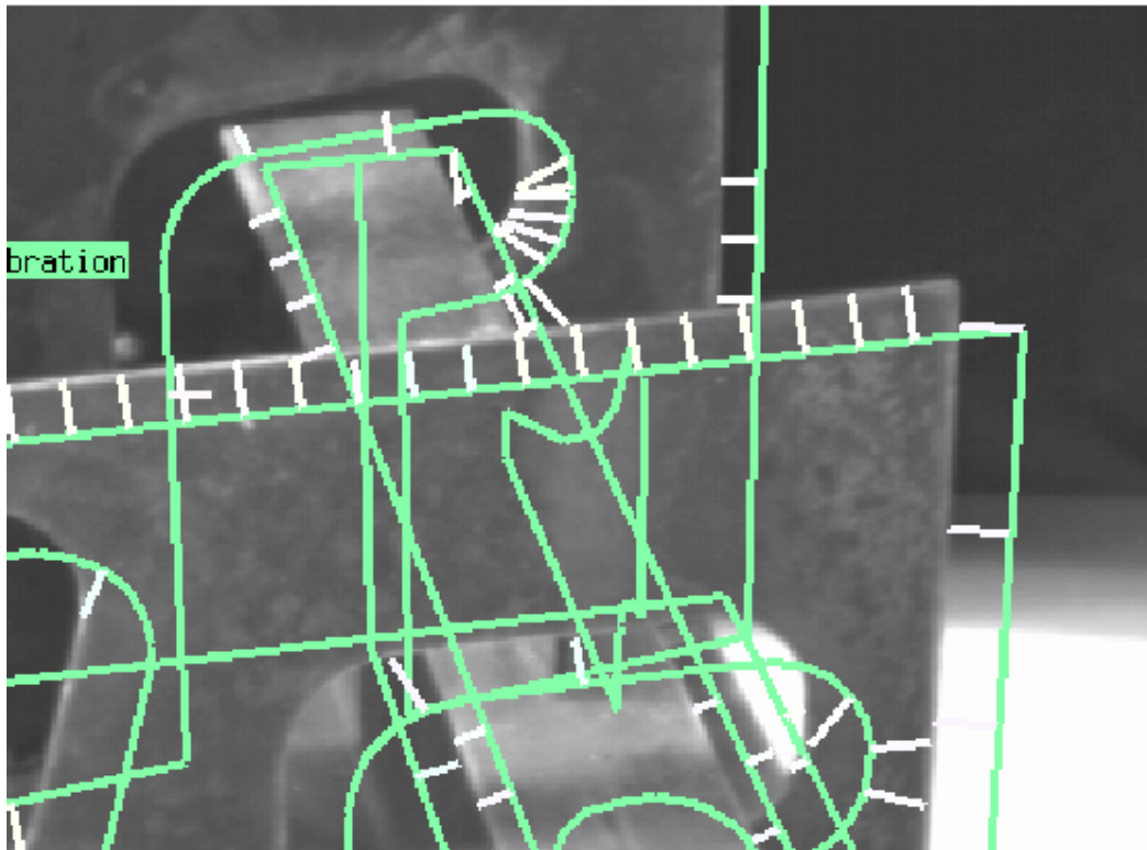
Figure 4: Points along model edges are associated with image contours – these model-point-to-image-contour correspondences are illustrated by short segments perpendicular to the model edges. Notice that a large number of model edges do not have image contours associated with them. The ability to restrict the number of matches to the most reliable ones is key to successful convergence of the tracking process.
