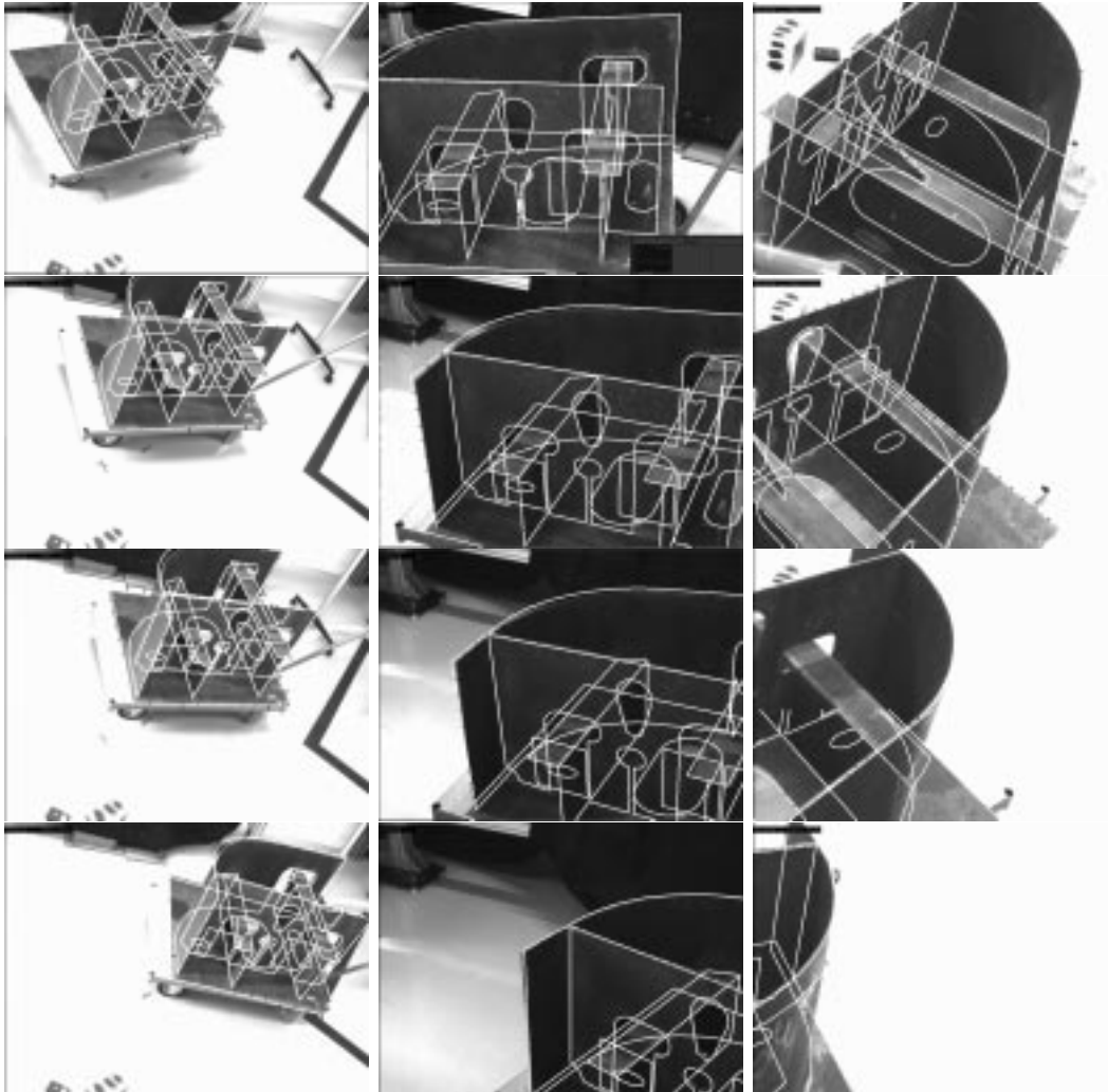
Figure 7: A tracking sequence. The object rotates and translates onto the floor. Notice that the three cameras have very different points of view.
