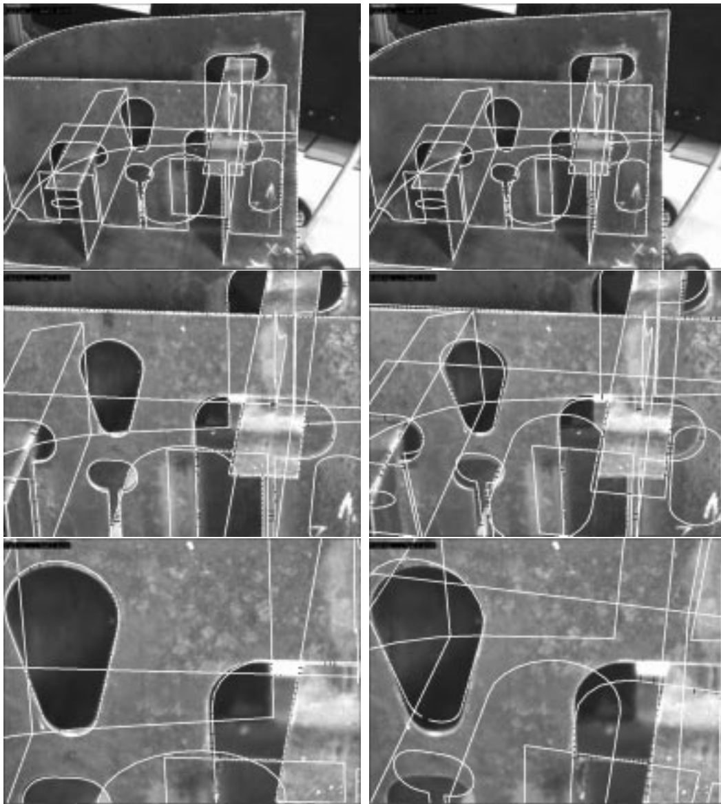
Figure 6: The effect of zooming in and zooming out can be taken into account by the tracker (left column). The right column shows the effect of tracking with fixed focal length: the zoom effect is compensated by variations in depth, but this compensation is far from being perfect.
