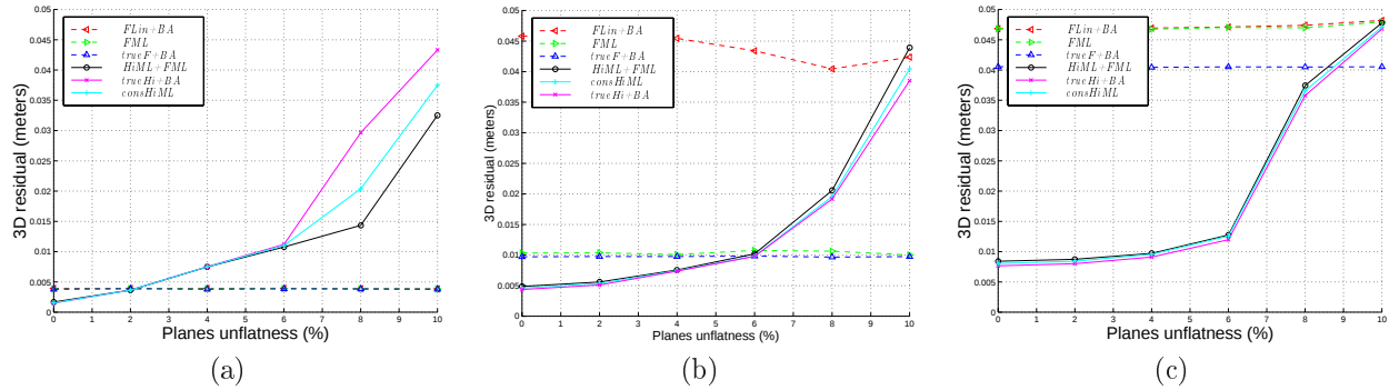
Figure 13: Comparison of the 3D residual E_3 for the estimators FLin+BA , FML , trueF+BA , HiML+FML , consHiML and trueHi+BA vs the unflatness of 3D planes for n=50 points per plane, 3 planes and a 3 pixel standard deviation noise. The distance cube/cameras \rho is (a) and (b): 3, (c): 11 and (d): 20 meters.
