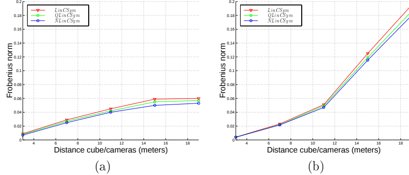
Figure 7: Comparison of the distance E_{\mathcal{F}} between the estimated homography \mathbf{H} and the true one \bar{\mathbf{H}} for the estimators LinCSym , NLinCSym and QLinCSym vs the distance plane/cameras \rho for a 1 pixel standard deviation noise, n=50 points per plane and 3 planes. (a): the true fundamental matrix is used and (b): the maximum likelihood estimate is used.
