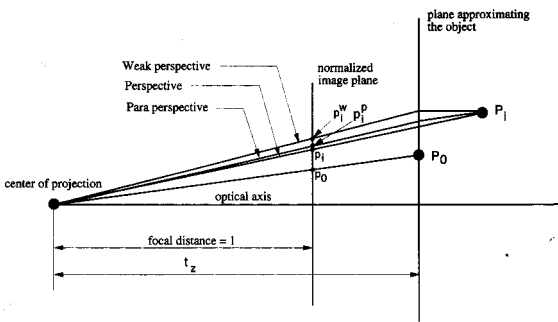
Figure 2. This figure shows p_0 , p_i —the perspective projections of two object points, P_0 and P_i , and p_i^w , p_i^p —the weak and paraperspective projections of P_i . The quality of the paraperspective projection depends on the angle between the line of projection of P_i and the line of projection of P_0 . Similarly, the quality of the weak perspective projection depends on the angle between the line of projection of P_i and the optical axis.
