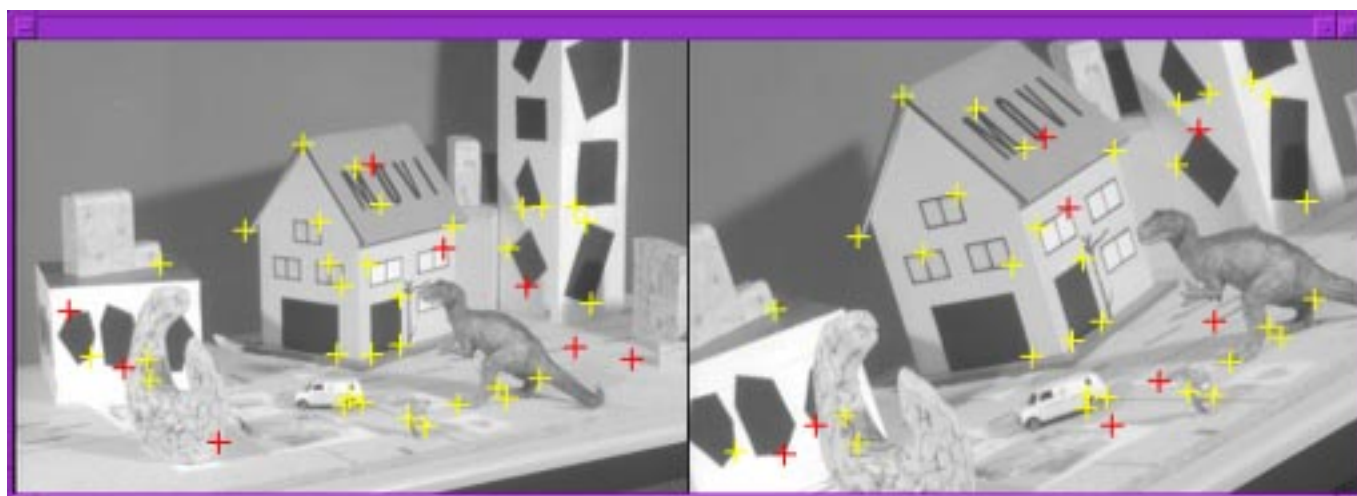
Figure 12: 80.0% correct matches
