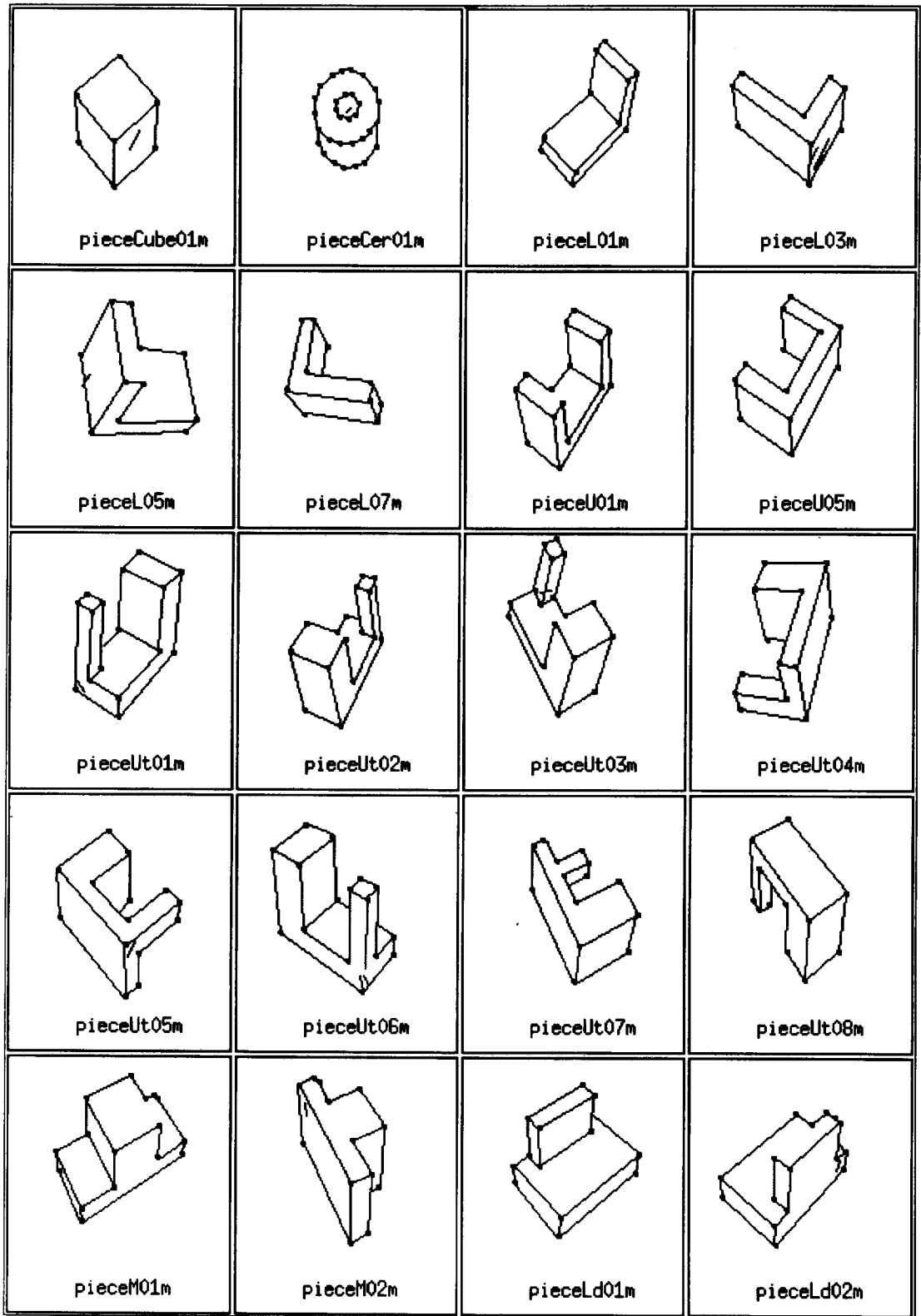
Fig. 9. The 20 graphs (lines and junctions) extracted from the previous images. These 20 graphs are decomposed into subgraphs (the decomposition is not shown) and stored in the hash-tables associated with the database.
