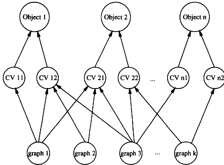
Fig. 2. The database has a three-layer structure: graphs, characteristic views and objects. An object may well have more than two characteristic views associated with it.
