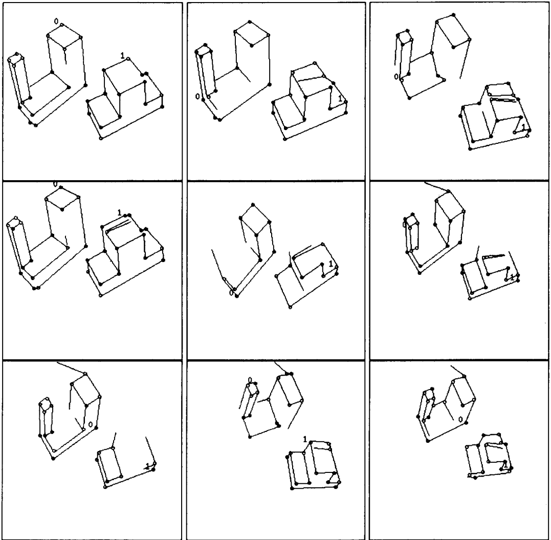
Fig. 11. The graphs extracted from the previous images. Notice that the noise corruption of these graphs varies extensively even if there is only a small change in camera position and orientation.
