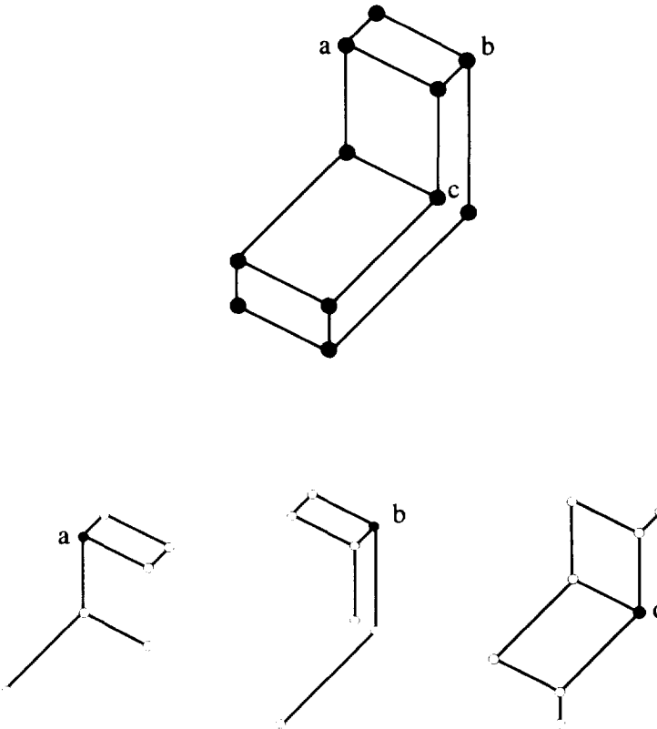
Fig. 3. An example of a characteristic view of an object and a few graphs extracted from this view.
