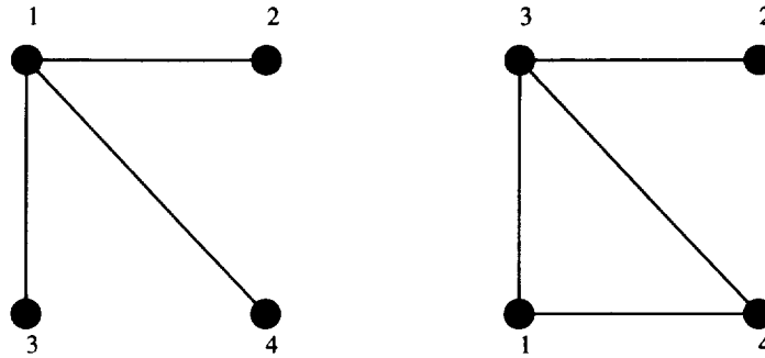
Fig. 1. These two graphs differ by one edge, but their associated second immanantal polynomials are quite different.
