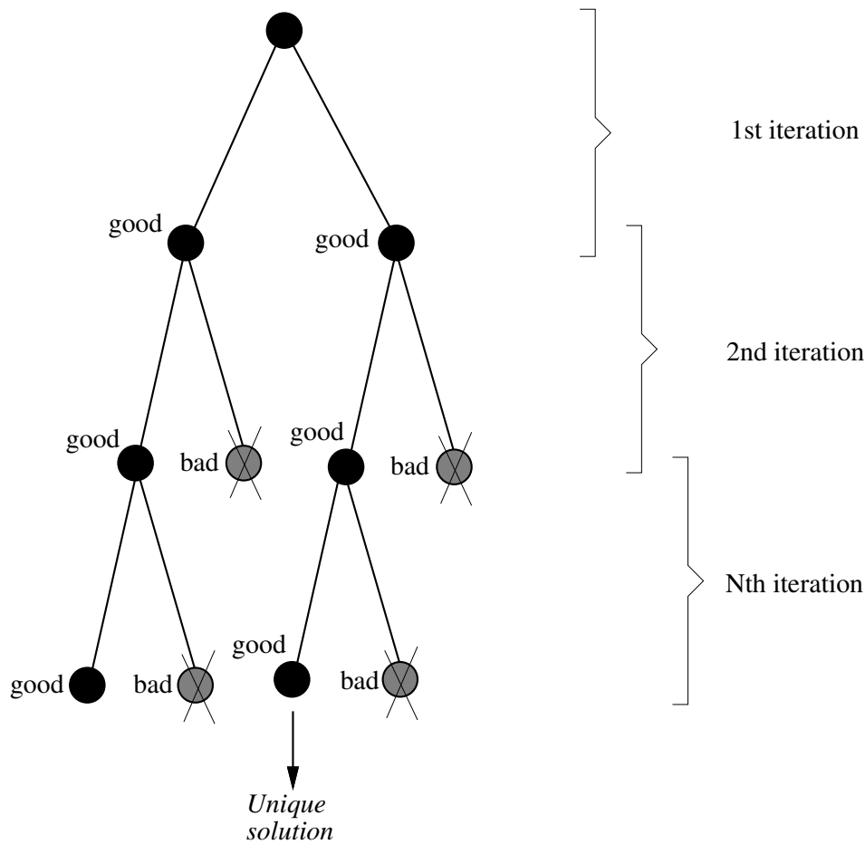
Figure 5: A binary tree search for selecting the best object pose when the object points are coplanar.
